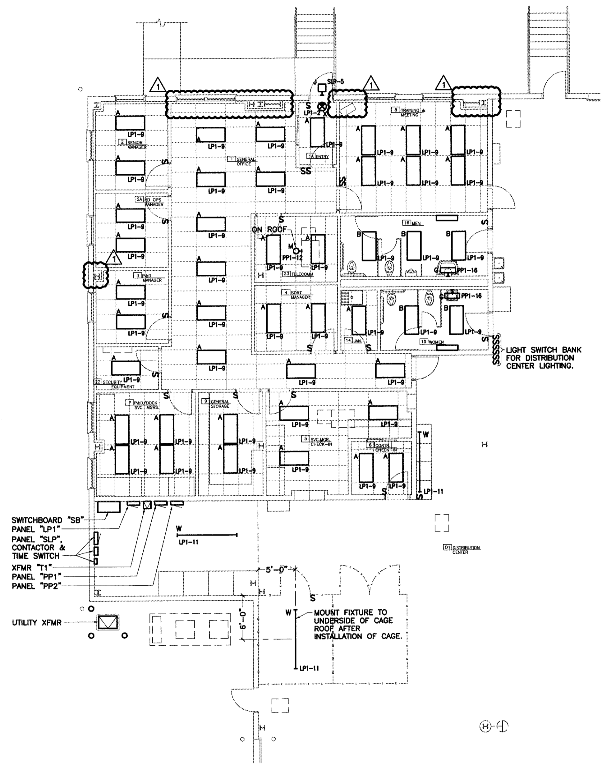
ENLARGED FLOOR PLAN - LIGHTING SCALE: 1/8"=1'-0"
