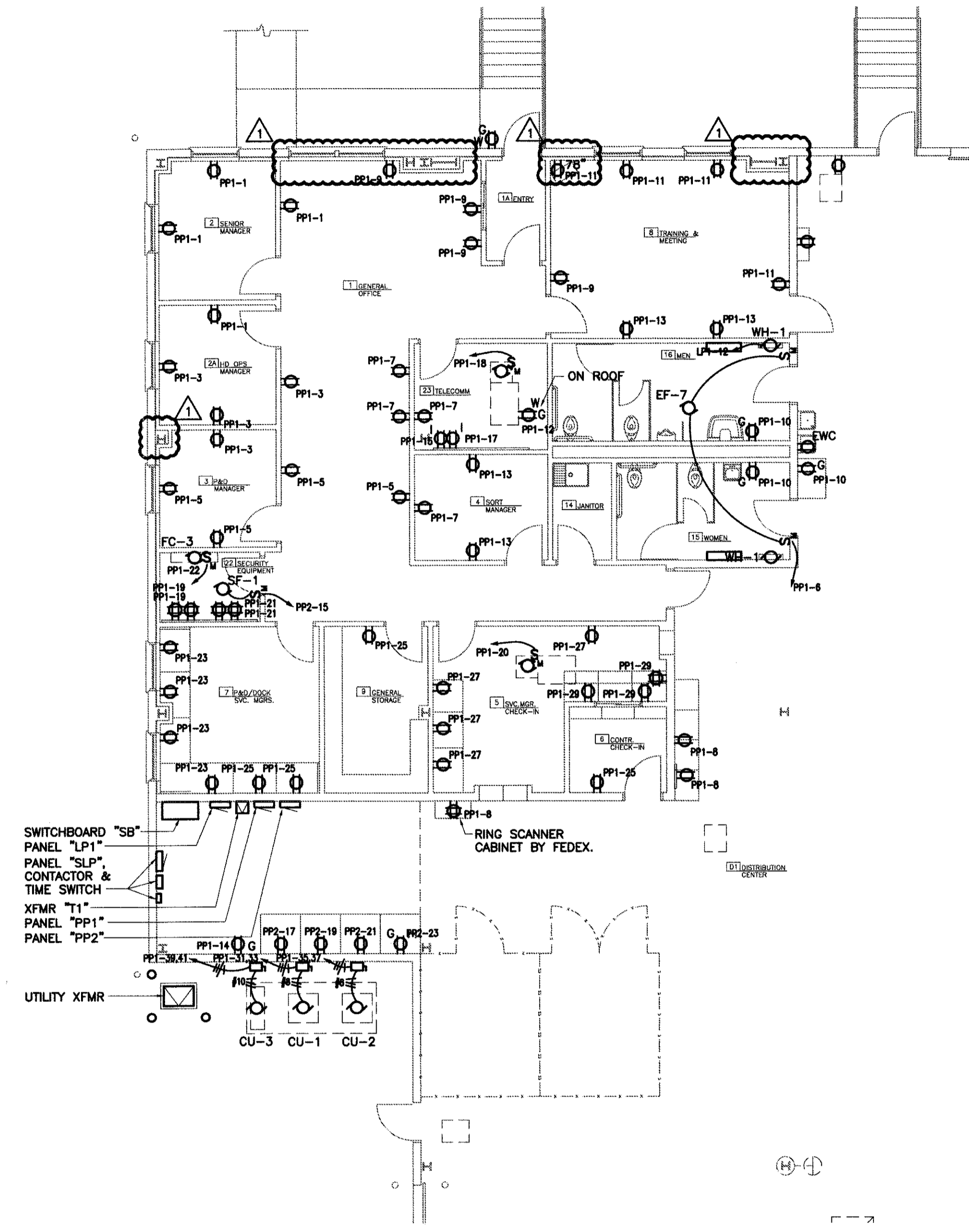
ENLARGED FLOOR PLAN - POWER SCALE: 1/8"=1'-0"
