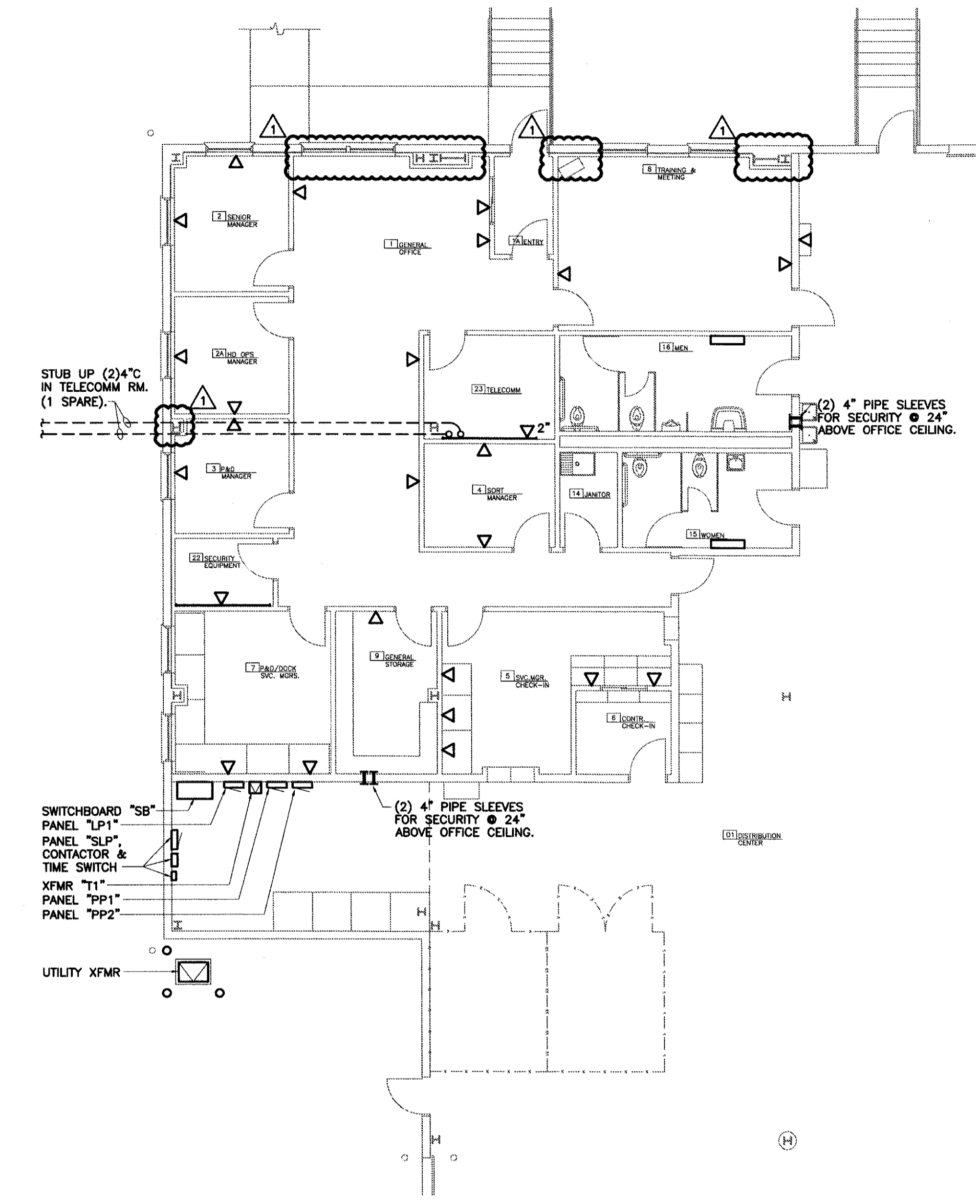
ENLARGED FLOOR PLAN - SYSTEMS SCALE: 1/8"=1'-0"
