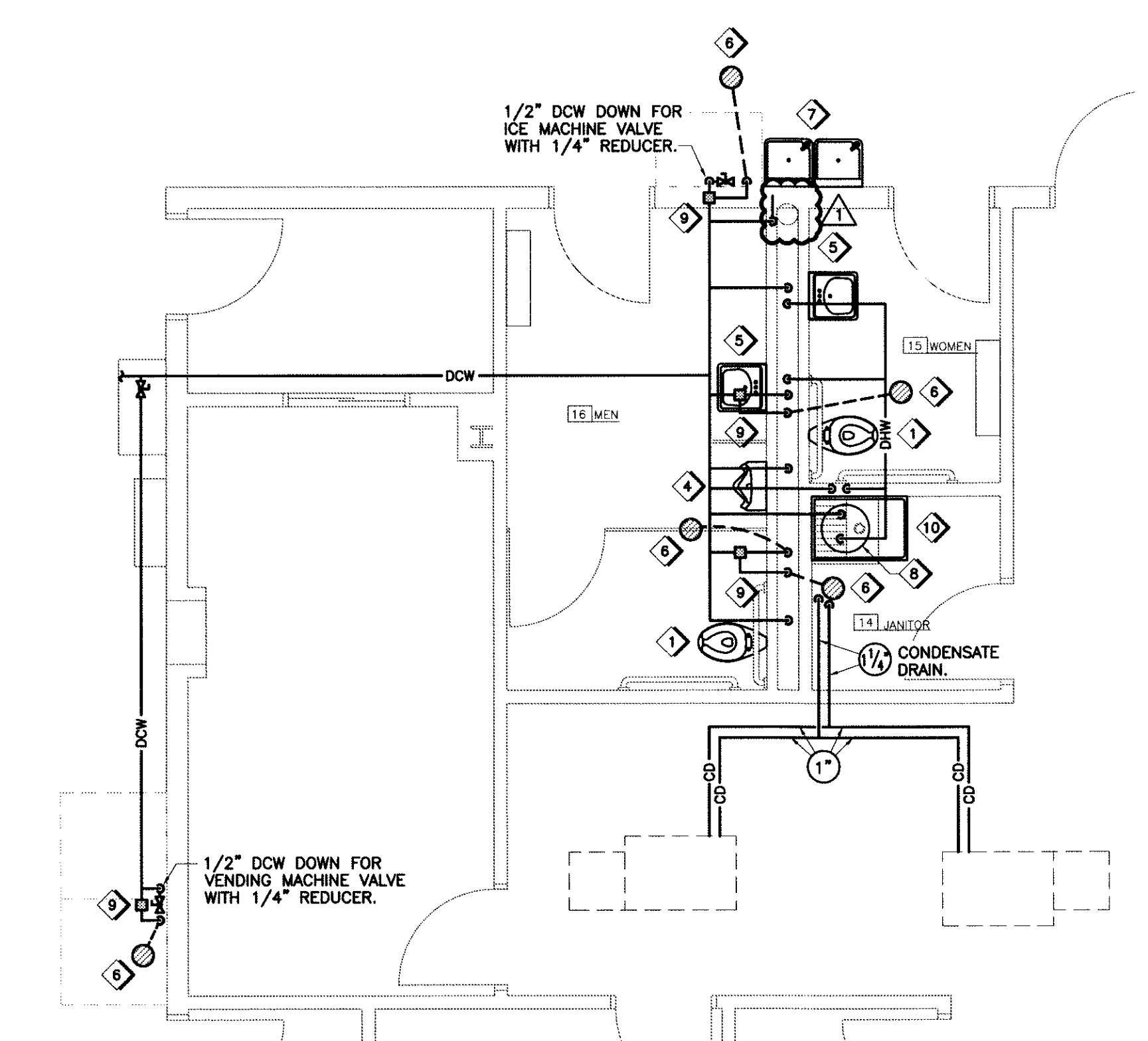
ENLARGED TOILET FLOOR PLAN - PLUMBING SCALE: 1/4"=1'-0"
