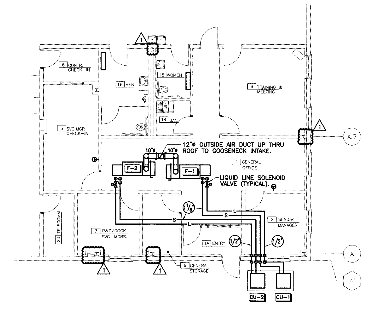
FLOOR PLAN - HVAC PIPING & O/A DUCTWORK SCALE: 1/8"=1'-0"
