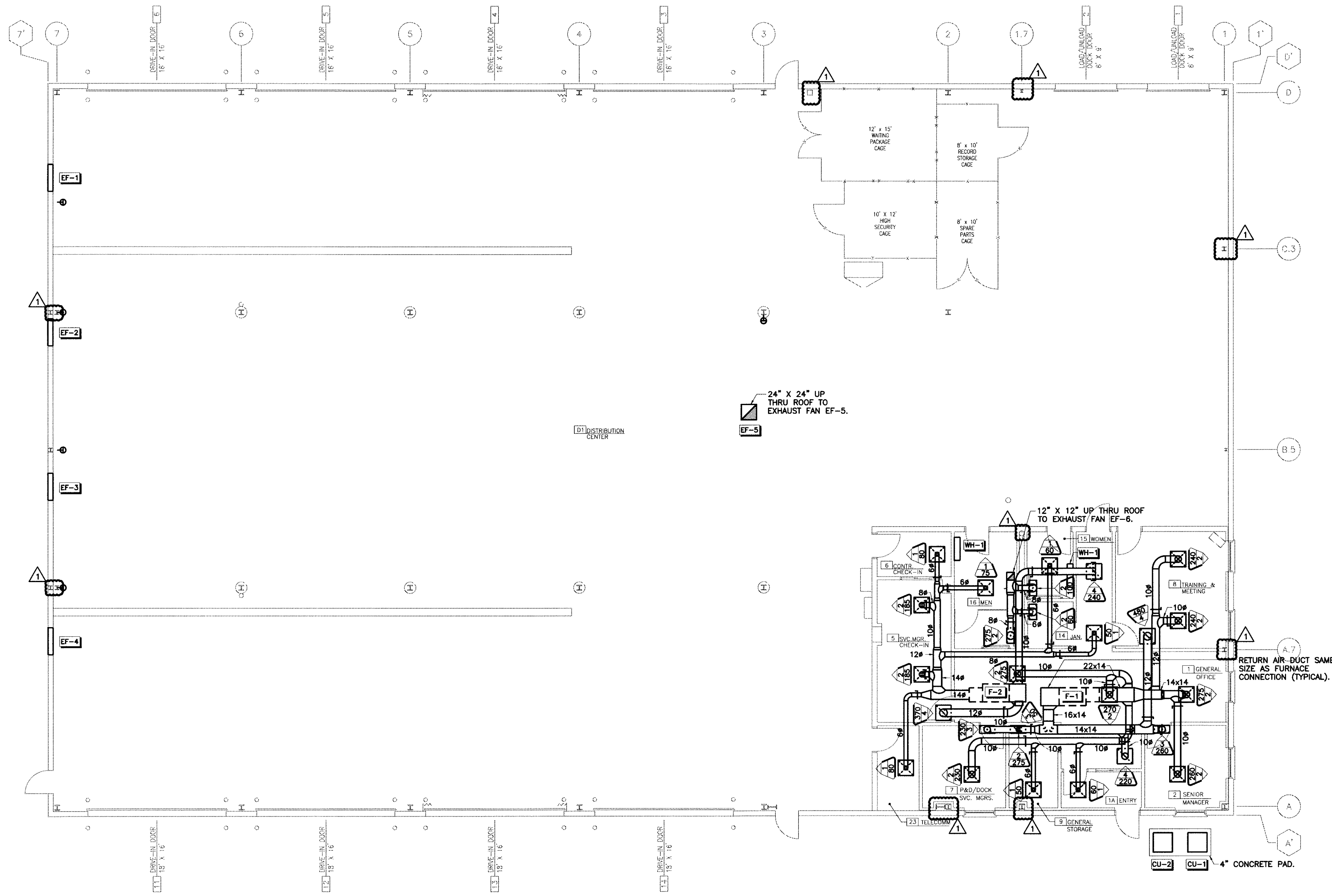
FLOOR PLAN - HVAC RETURN & SUPPLY DUCTWORK SCALE: 1/8"=1'-0"
