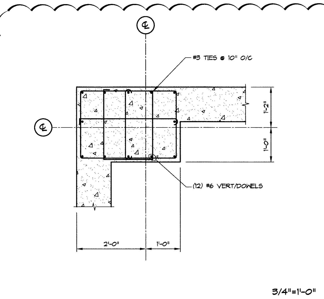
5 PIER P5
